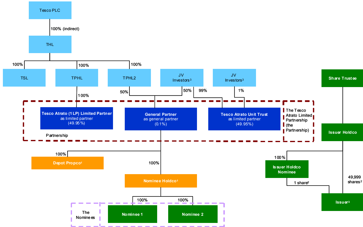
FIGURE 1: OWNERSHIP STRUCTURE
