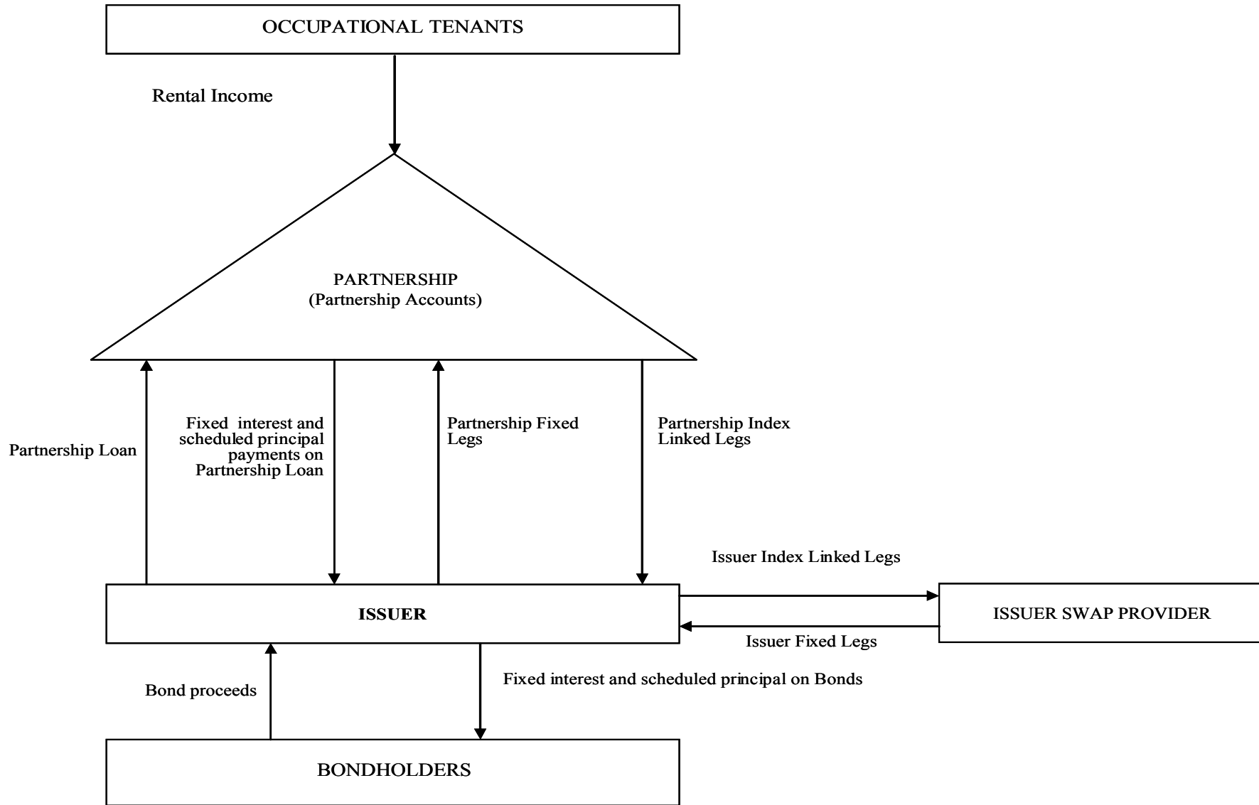
FIGURE 2: TRANSACTION STRUCTURE
